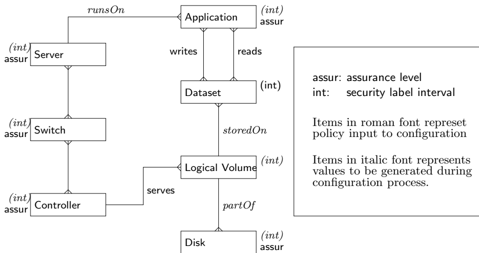
Figure 1. The Structure of a SAN.
